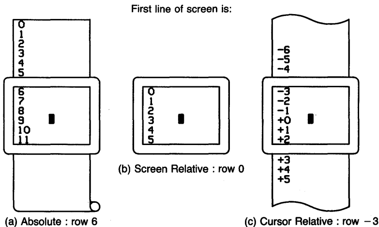
Figure 3. Row Addressing
