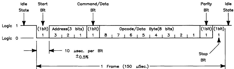
Bit Format for a Frame
